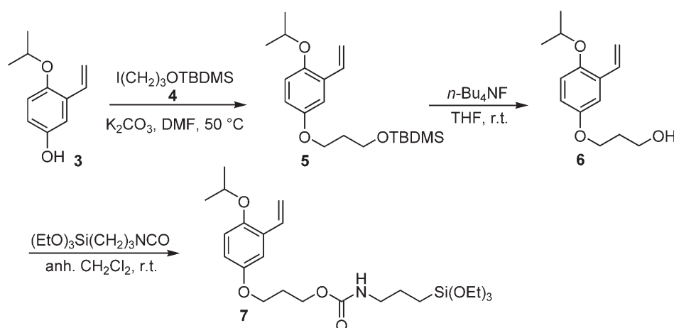
Scheme 1. Preparation of the monosilylated Hoveyda-type monomer 7 .
