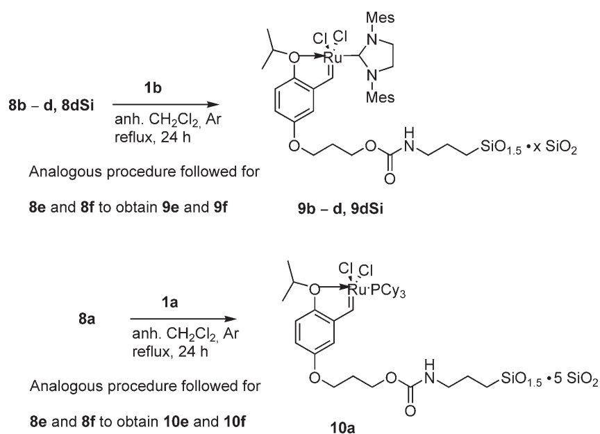
Scheme 3. Preparation of ruthenium heterogeneous catalysts 9a–f , 9dSi , 10a , 10e and 10f from the corresponding materials 8 .
