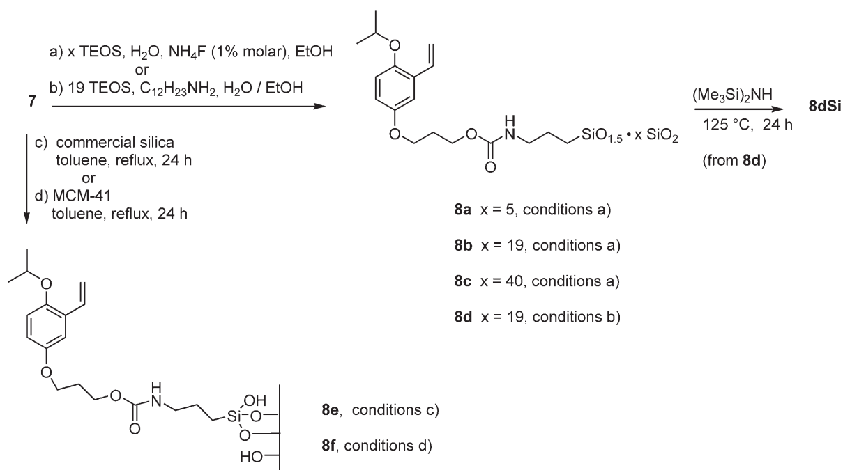
Scheme 2. Preparation of hybrid silica materials 8a–f and 8dSi from 7 .
