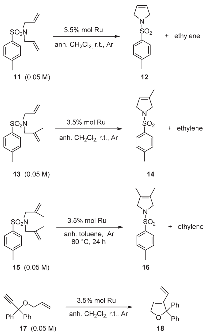
Scheme 4. Diene and enyne metathesis reactions tested with recyclable catalysts 9 and 10 .
