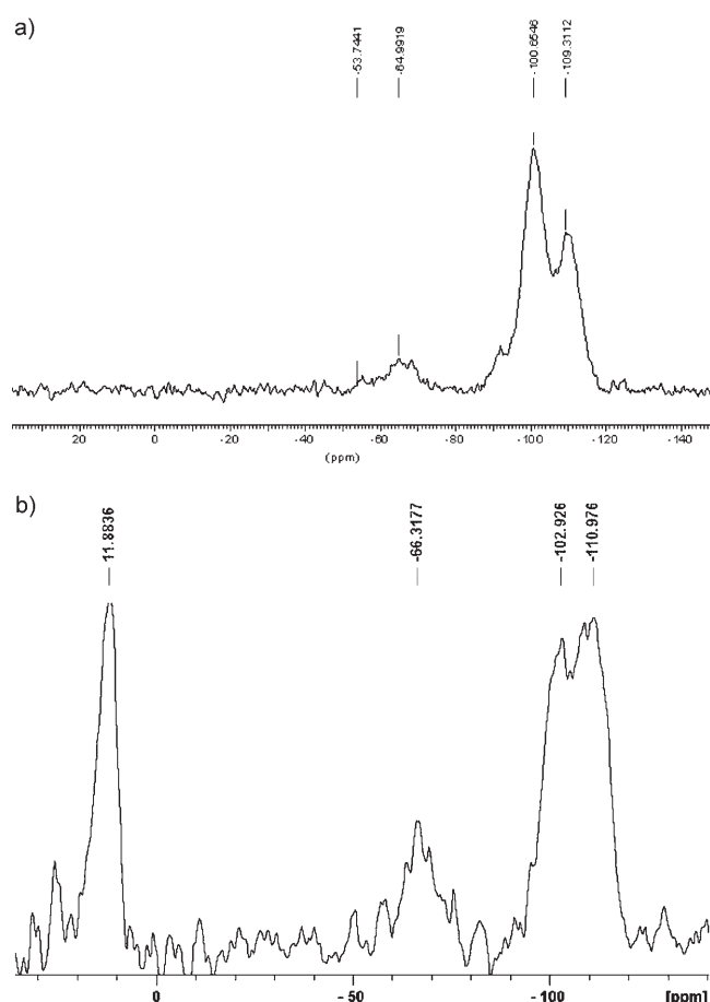
Figure 2. Solid state CP-MAS NMR: a) ^{29}\text{Si} of 8d and b) ^{29}\text{Si} of 8dSi .
